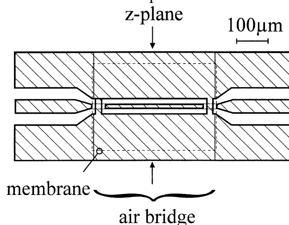
Fig. 1: Geometrical configuration of the CPW structure.
