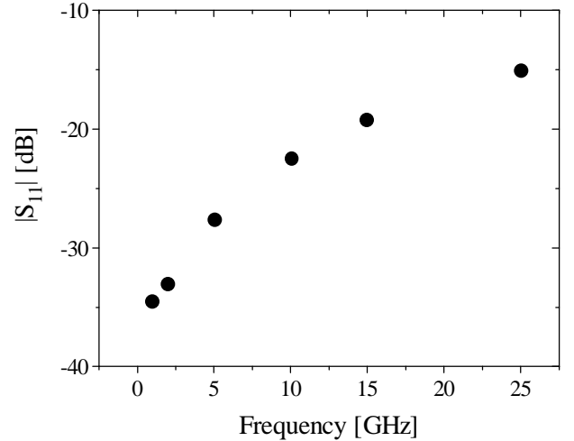
Fig. 4: Simulated results for the reflection coefficient for CPW on a membrane.
